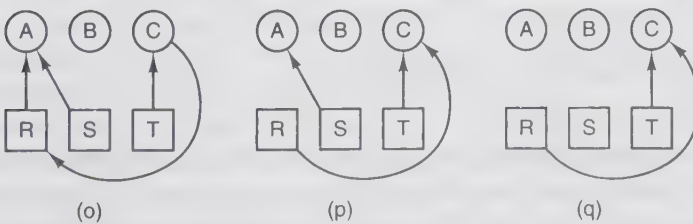
Figure 3-10. An example of how deadlock occurs and how it can be avoided.
