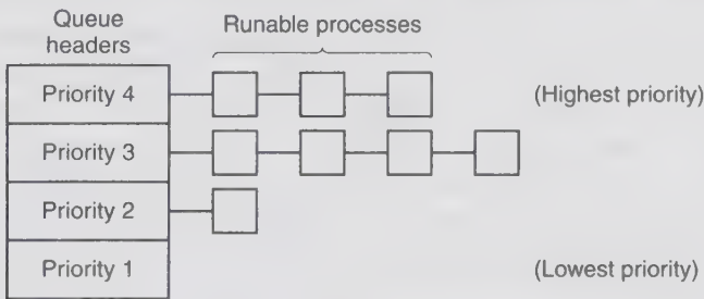
Figure 2-27. A scheduling algorithm with four priority classes.
