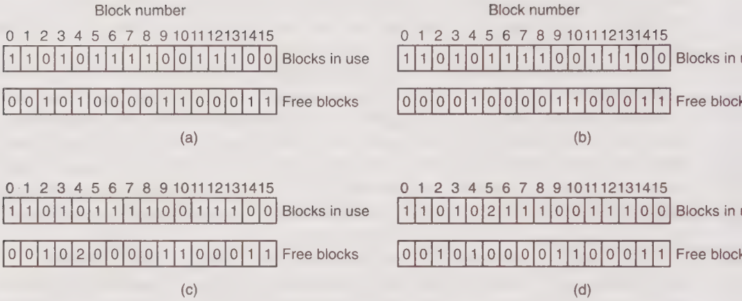
Figure 5-19. File system states. (a) Consistent. (b) Missing block. (c) Duplicate block in free list. (d) Duplicate data block.
