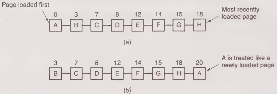
Figure 4-14. Operation of second chance. (a) Pages sorted in FIFO order. (b) Page list if a page fault occurs at time 20 and A has its R bit set. The numbers above the pages are their loading times.
