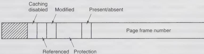
Figure 4-11. A typical page table entry.
