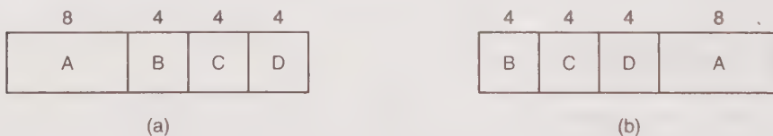
Figure 2-24. An example of shortest job first scheduling. (a) Running four jobs in the original order. (b) Running them in shortest job first order.
