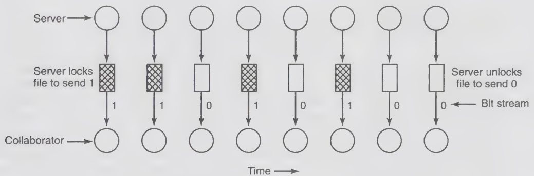
Figure 5-32. A covert channel using file locking.
