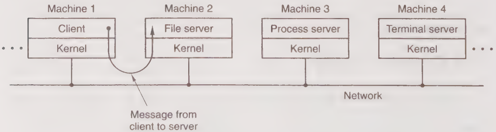
Figure 1-21. The client-server model in a distributed system.
