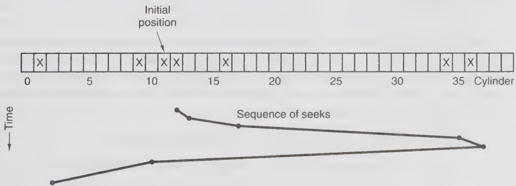
Figure 3-22. The elevator algorithm for scheduling disk requests.
