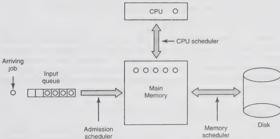
Figure 2-25. Three-level scheduling.
