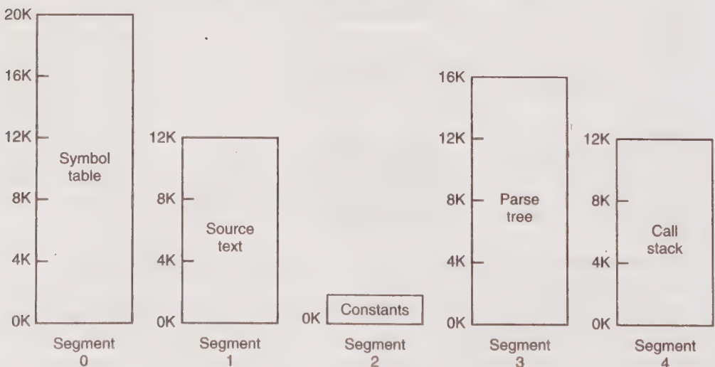
Figure 4-22. A segmented memory allows each table to grow or shrink independently of the other tables.
