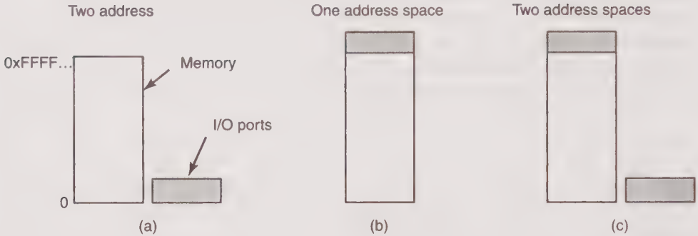
Figure 3-3. (a) Separate I/O and memory space. (b) Memory-mapped I/O. (c) Hybrid.
